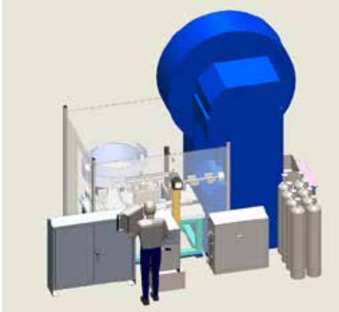
A work cell with an automated feed to a hot header for large bolts. Ambrell works with expert integrators to provide a turnkey solution to customers.
