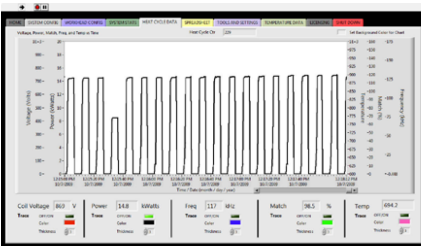
A screen view of eVIEW software monitoring a fastener hot heading process showing one part heating to only 750 °C instead of the correct process temperature of 900 °C.
